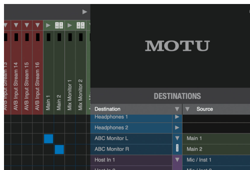
Figure 5-9: Routing host computer (DAW) output to the ABC Monitor channels (via the 10pre's built-in mixer).
