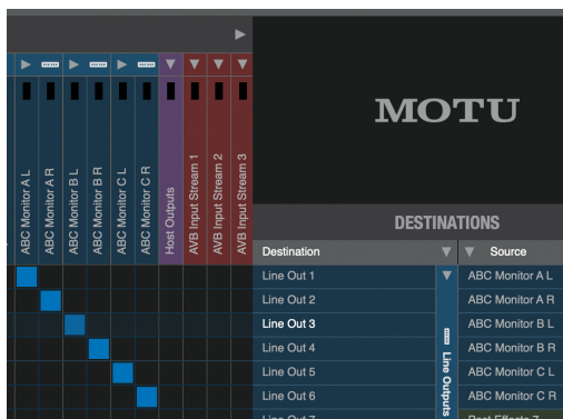
Figure 5-7: Routing the A/B/C Monitor source signals to their respective outputs. In this example, Monitor A is routed to Line Outs 1-2, Monitor B is routed to Line Outs 3-4 and Monitor C is routed to Line Outs 5-6. This is only an example; you can use any outputs you wish (analog, digital or even network channels).
