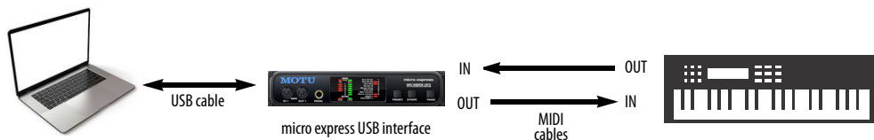
Figure 3-1: An example of connecting a single MIDI device to a MOTU micro express interface. Connect the device’s MIDI OUT and MIDI IN ports to the interface.
